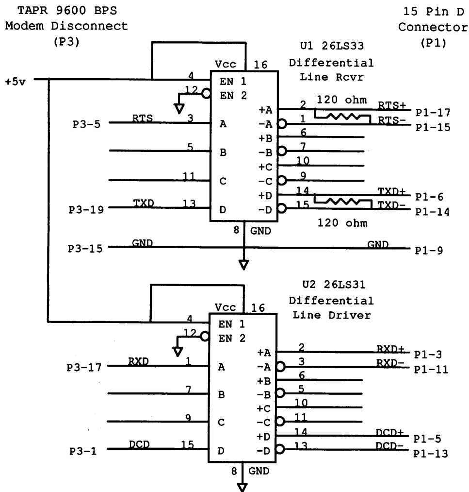
Schematic Diagram for TAPR 9600 bps Modem Daughter Board
