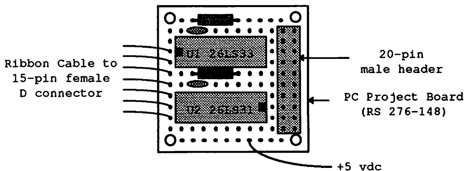
RS-422 Interface Daughter Board for TAPR 9600 bps Modem (drawing is not to scale)
